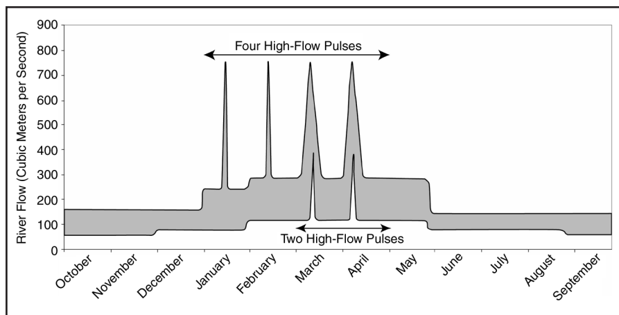
Figure 2: Instream flow recommendations for the Savannah River were specified for three types of water years (dry, average, wet). The shaded band reflects desired flow conditions. In dry years, water managers will follow the lower end of the band range; during wet years, flows will be closer to the upper band limit.
